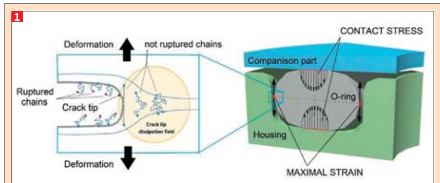
Fig. 1. Visualization showing the typical deformation of a crack tip and association of ruptured and non-ruptured chains at the vicinity of the crack tip for a seal application.
